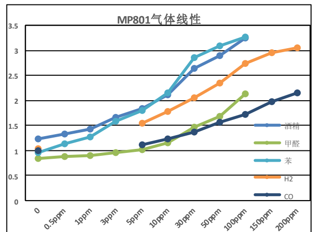
Fig6. Linearity curve
