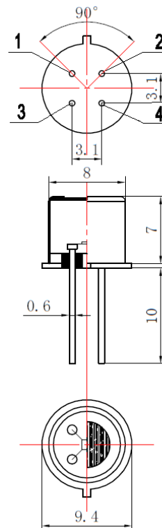
Fig1. Sensor Structure
