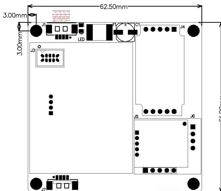
Fig 3: Mounting dimension
