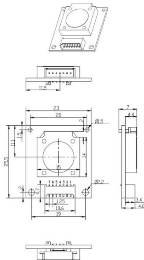
Fig. 1: structure
