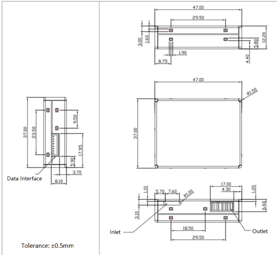
Fig4. Sizes
