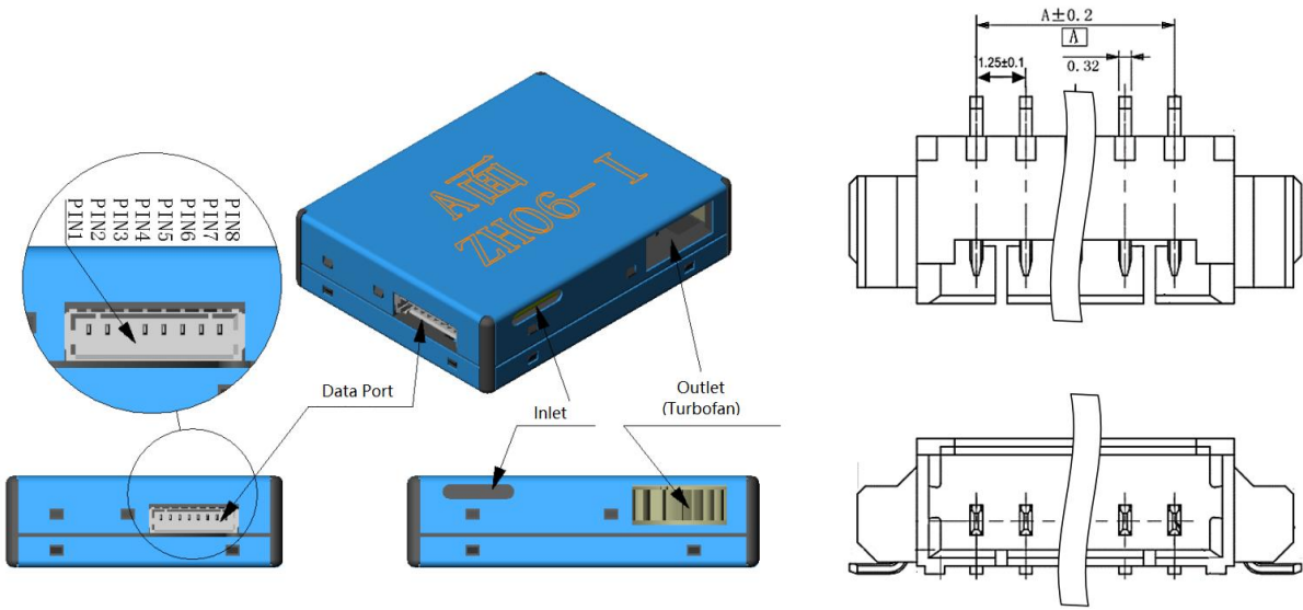
Fig1. Pin Order
